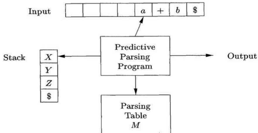
Figure 2.2: Model for table-driven parsing
